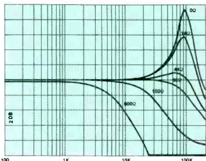
Figure 2. Frequency response of a 1,000-foot cable with various values of source impedance. The flattest response results in a source impedance of approximately 60 \Omega .
