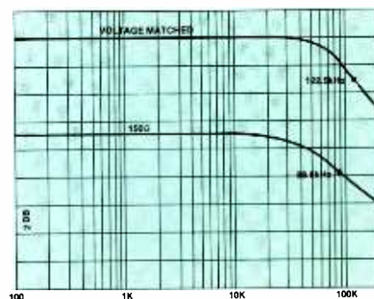
Figure 4. Comparison of frequency response for a 1,000-foot cable when used in voltage-matched and 150 \Omega matched systems. Markers represent the -3dB points.
