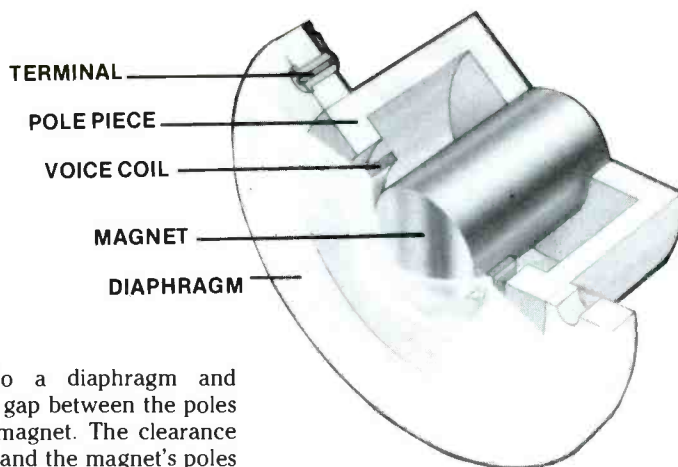
A basic dynamic microphone element.
