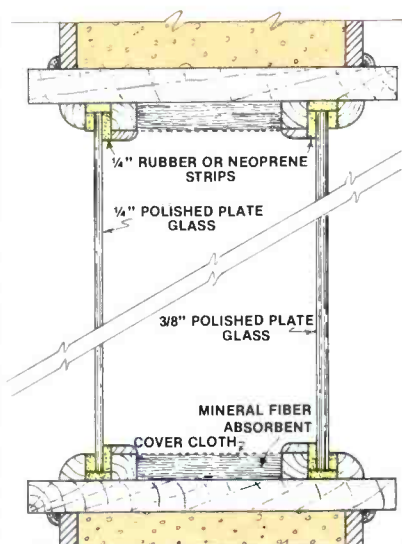
Figure 2. Typical control room window construction.
