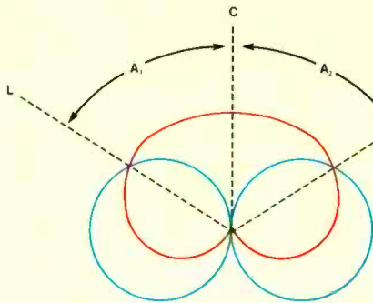
M-S pattern overlay. Angles A_1 and A_2 are always equal and will vary depending on the relative gain of the M vs. S microphones.
