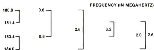
Figure 10. A sample calculation of IM compatibility for an event using four wireless microphones.
