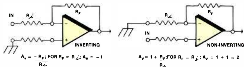
Figure 13. Inverting and non-inverting operational amplifiers.
