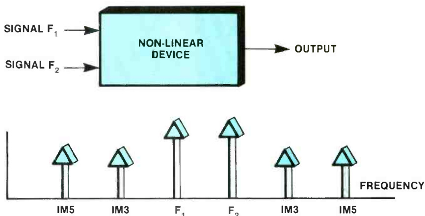
Figure 9. Intermodulation is produced when two or more signals combine in a non-linear device.
