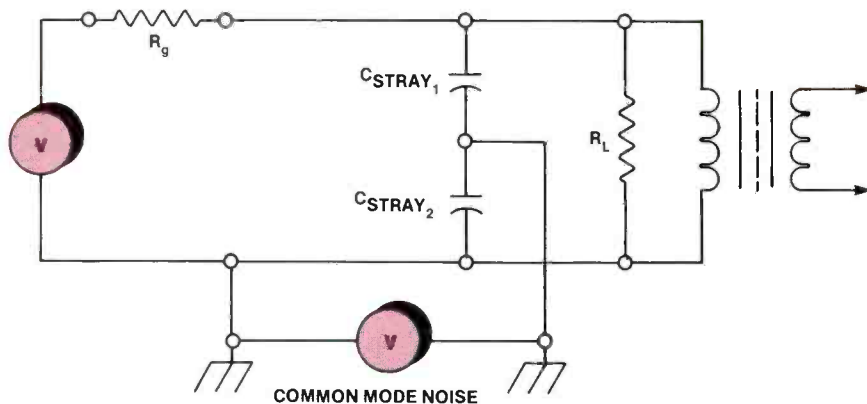
Figure 7. Capacitive leakage paths develop when high frequencies are present. These paths are represented by C_{\text{stray } 1} and 2 .
